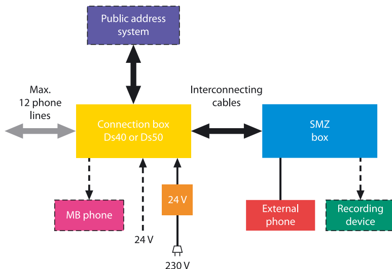
Block diagram
